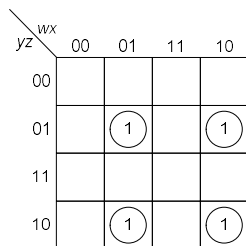
(a) Map of f(x,y,z) = \sum(5,6,9,10) = w'xy'z + wx'y'z + w'xyz' + wx'yz'
