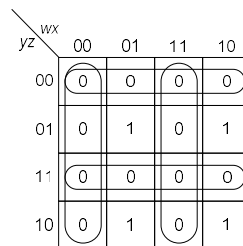
(b) Map of f(x,y,z) = \prod(0,1,2,3,4,7,8,11,12,13,14,15) = (y+z)(y'+z')(w+x)(w'+x')
